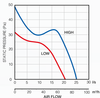
QuietAir QT100
