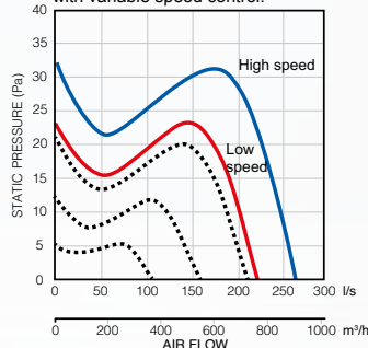
QuietAir QT150
