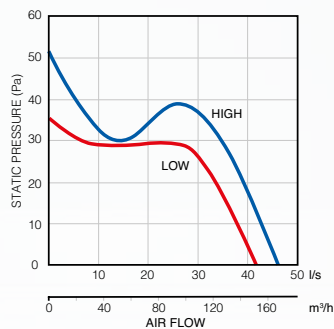
QuietAir QT120
